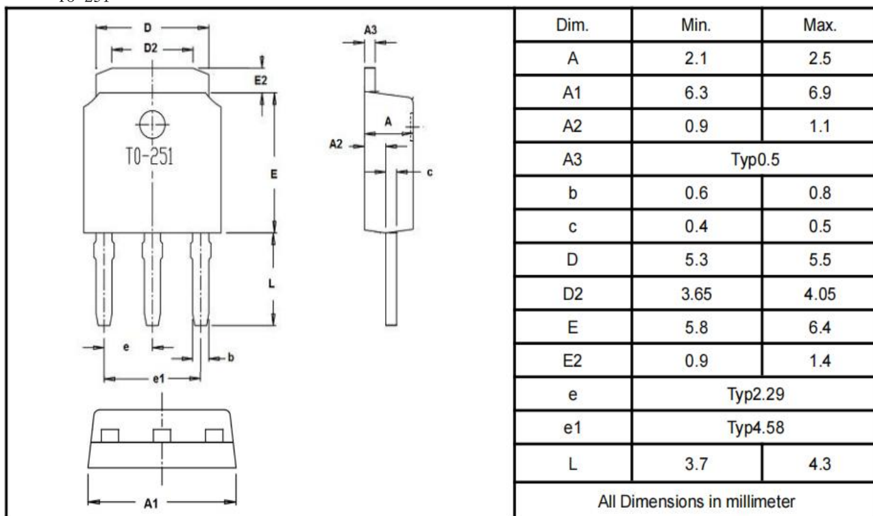
TO-251
