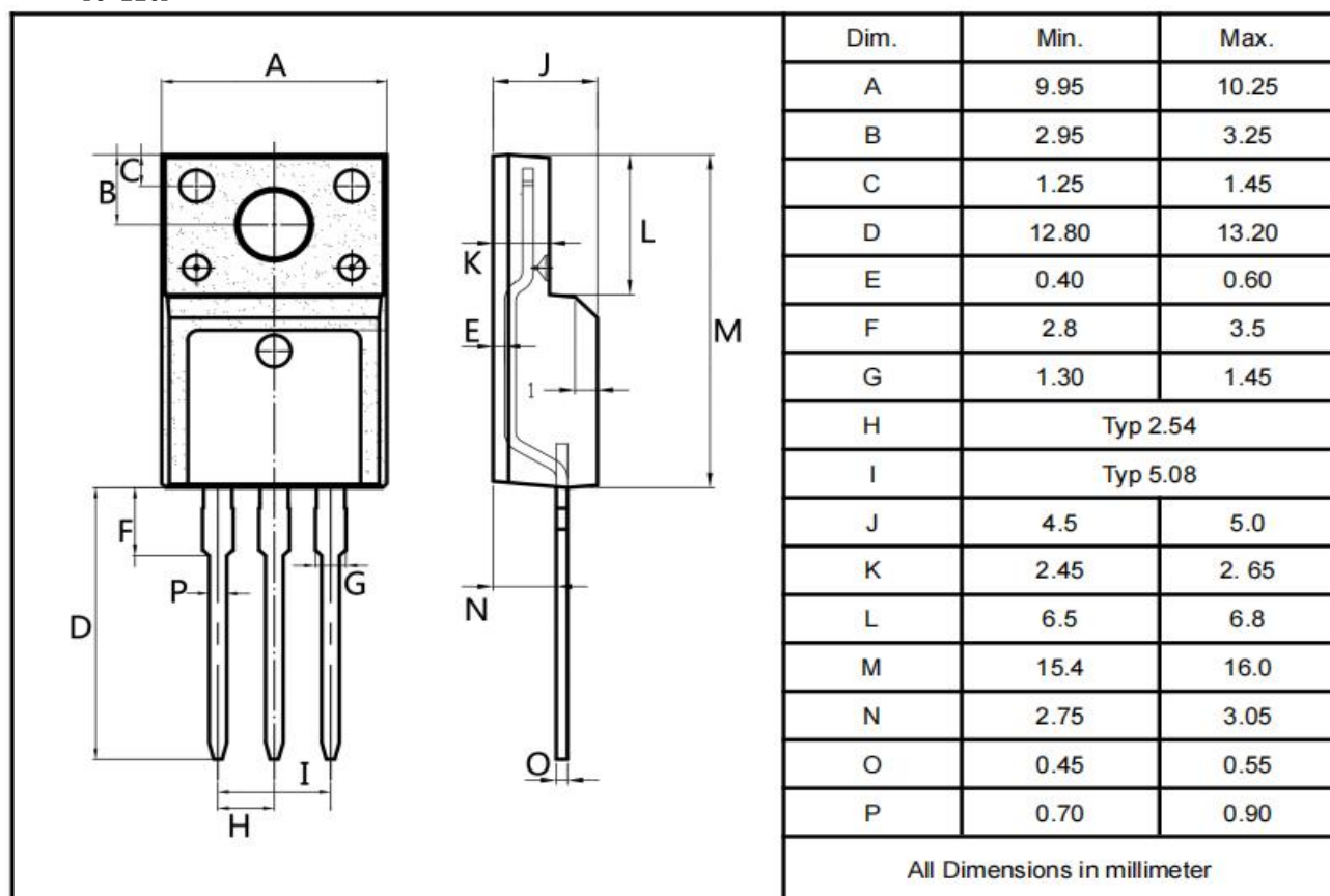
TO-220F
