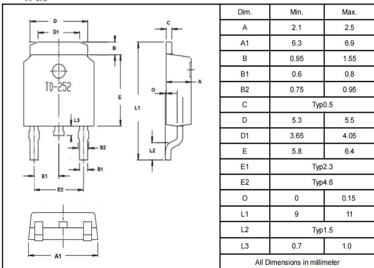
TO-252
