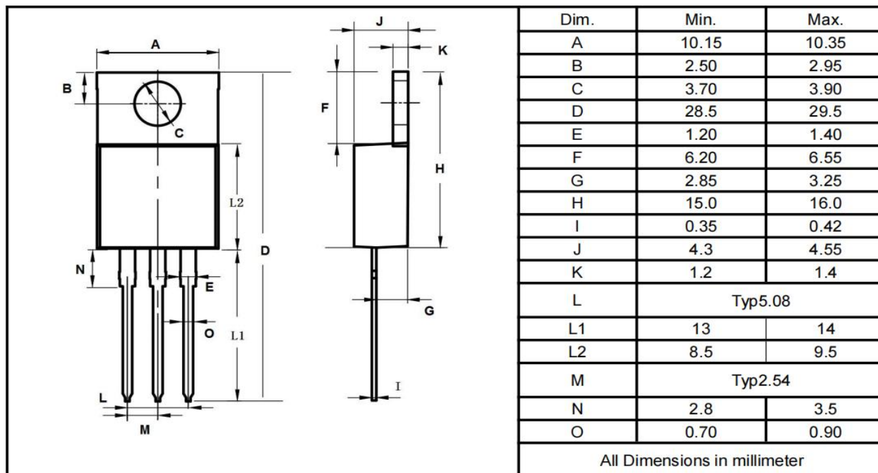
TO-220AB
